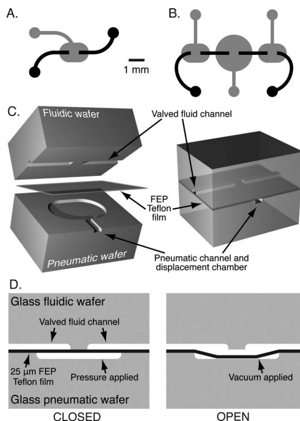
Fig. 2 Mask designs of a monolithic membrane valve (A) and pump (B); fluidic features are black, pneumatic features are gray, and small circles indicate the locations of drilled fluidic or pneumatic access holes. (C) Exploded and assembled illustrations of a single FEP valve. In the cross-sectional view of a single valve (D), the FEP film seals against the gap in the fluid channel when the valve is closed. Applying vacuum to the displacement chamber pulls the film away from the fluidic wafer and opens the valve.
