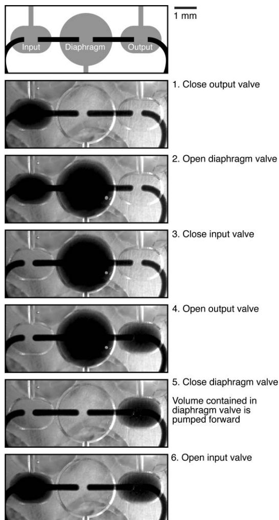
Fig. 3 Photographs of dye in a 340 nL FEP Teflon pump at each of the six steps in a single pump cycle. At the optimal actuation rate for this pump, this cycle repeats every 90 ms and pumps 1.1 \mu\text{L s}^{-1} .
