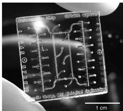
Fig. 1 Photograph of an Autosampler Chip containing 22 FEP Teflon monolithic membrane valves. The Autosampler Chip can deliver extremely caustic piranha solution (concentrated sulfuric acid and hydrogen peroxide) to clean an off-chip sensor without causing any detectable damage to the chip or its valves. 23
