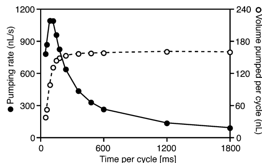
Fig. 6 Pumping rate and volume pumped per cycle as a function of actuation time for a 340 nL FEP Teflon diaphragm pump.
