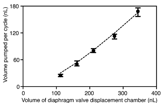
Fig. 5 Mean volume pumped per cycle by FEP Teflon pumps with diaphragm valves of five different volumes. The dashed line shows volumes predicted by modeling the volume inside the open diaphragm valve as a frustum of a cone (see text). Error bars show the range of individual pumping rates for the six pumps of each size measured.
