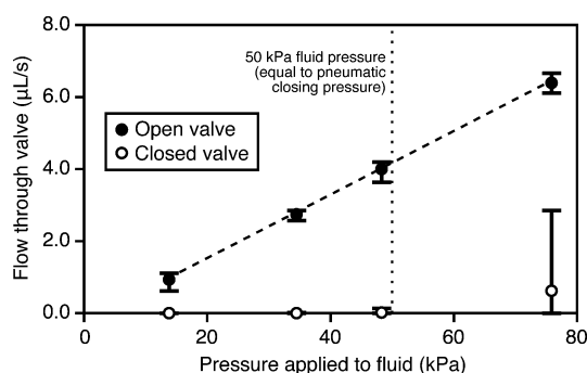
Fig. 4 Mean flow through ten open and closed FEP Teflon valves as a function of upstream pressure applied to the fluid. Flow through the open valve increases linearly with pressure, while flow through the closed valve is negligible at pressures below the pneumatic pressure used to hold the valve closed (50 kPa). Error bars show the range of individual flow rates for the ten valves measured.
