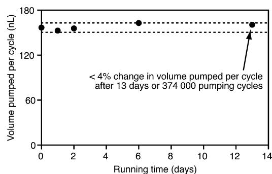
Fig. 7 Volume pumped per cycle by a 340 nL FEP diaphragm pump after 0, 1, 2, 6, and 13 days of continuous pumping. The dashed lines show the region of \pm 4\% change from the original value.
